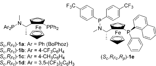
FIGURE 1. Representative structures of BoPhoz-type ligands 1a–e for asymmetric hydrogenation.
